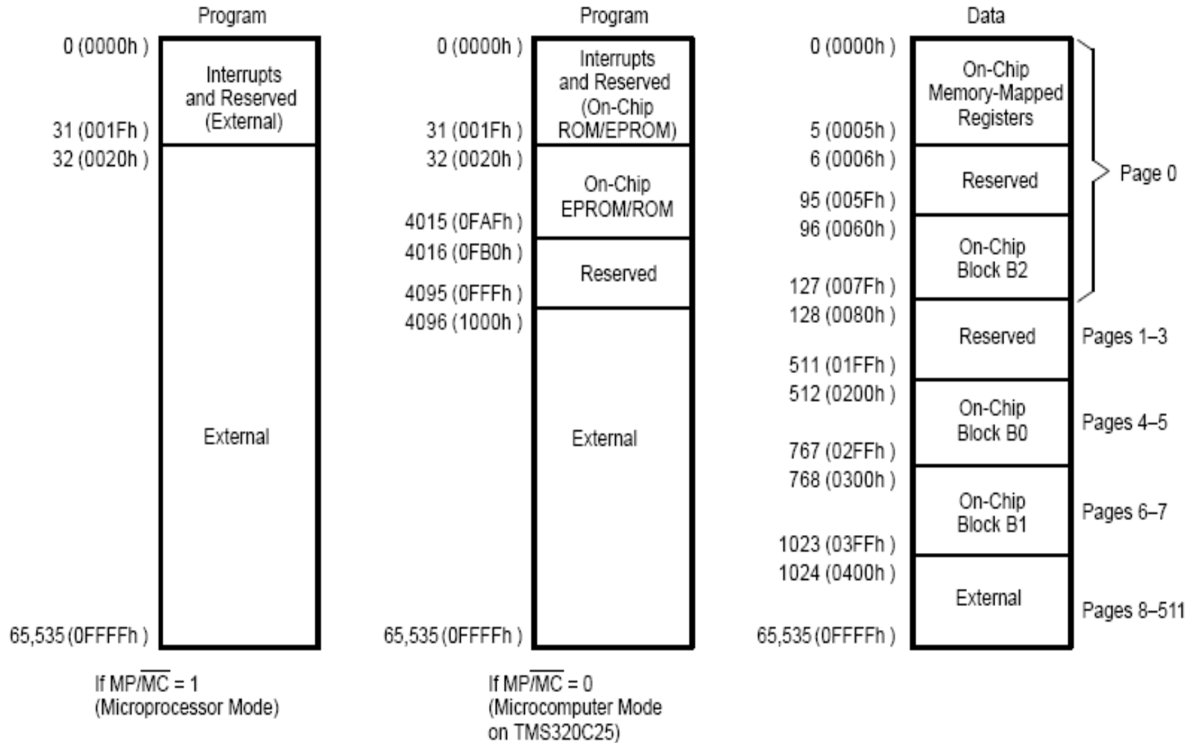
(a) Memory Maps After a CNFD Instruction
